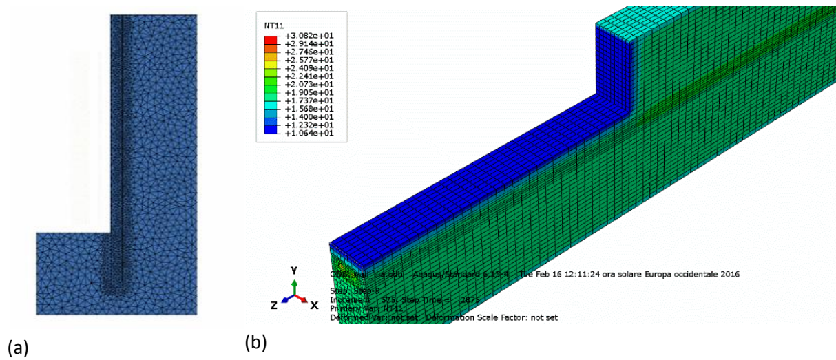
Figure 1 - (a) Feflow model and (b) Abaqus model.
